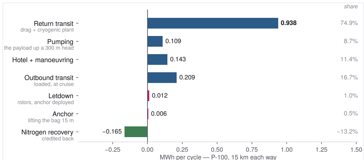
Figure 5. The reference ship's cycle ledger, printed from the model rather than transcribed. Three quarters of it is the return leg; the anchor is the smallest positive line and it is the reason the letdown is the second smallest.
