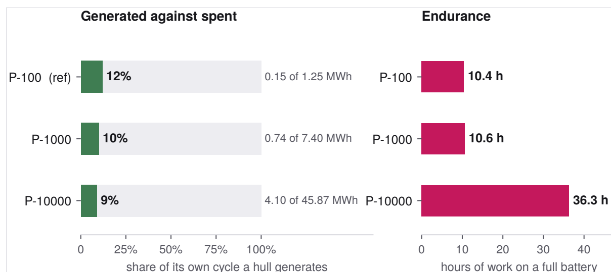
Figure 7. What each hull spends against what its skin makes, and how long a full battery lasts.
