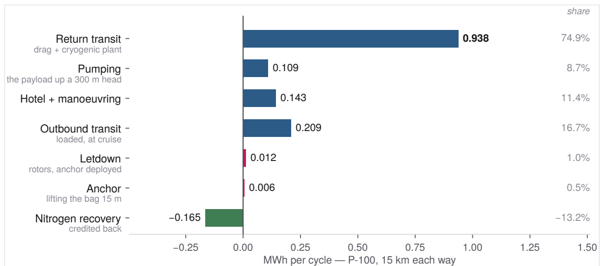
Figure 4. The reference ship's cycle ledger, printed from the model. Three quarters of it is the return leg; the mechanism that closes the descent costs half a per cent.
