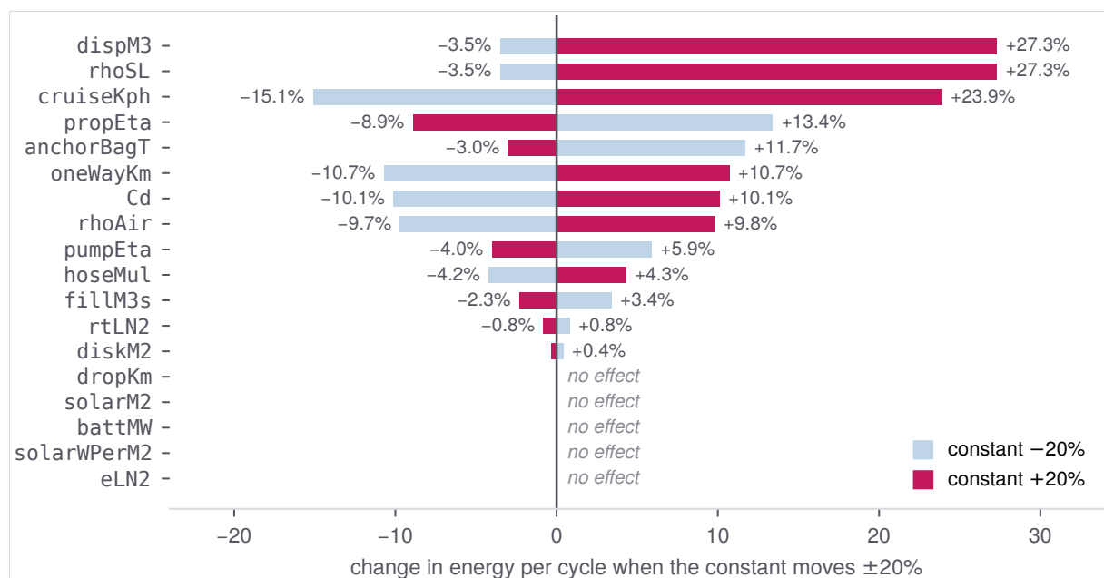
Figure 6. Every constant moved \pm 20\% , generated rather than transcribed. Where the model's uncertainty actually lives: aerodynamics and speed, not lift.
