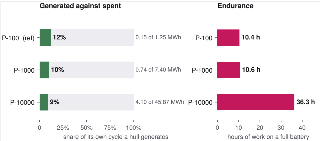
Figure 5. Spend against generation, and endurance on a full battery. This is the project’s central public conclusion and it is not a favourable one.
