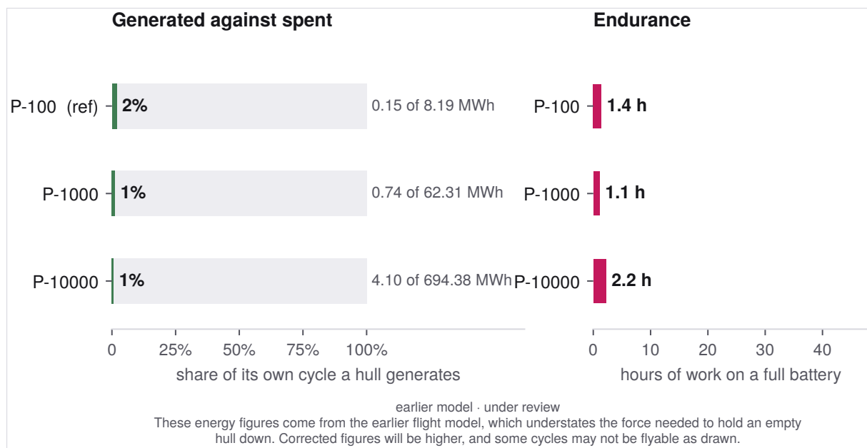
Figure 5. Spend against generation, and endurance on a full battery. This is the project’s central public conclusion and it is not a favourable one.
