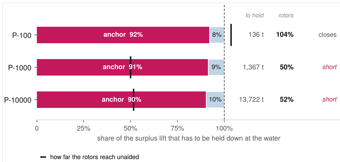
Figure 3. The problem the anchor solves. The bar is what has to be held down at the water; the tick is how far the rotors reach unaided.
