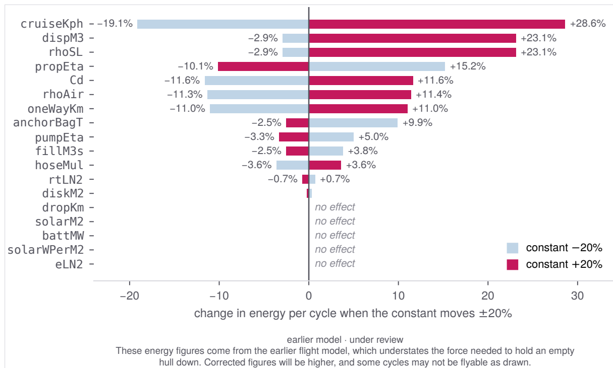
Figure 8. Every constant moved \pm 20\% , measured rather than asserted. The top of the table is aerodynamics and speed; the two constants corrected on 2026-08-09 now move the headline by 0.8% and 0.0%.
