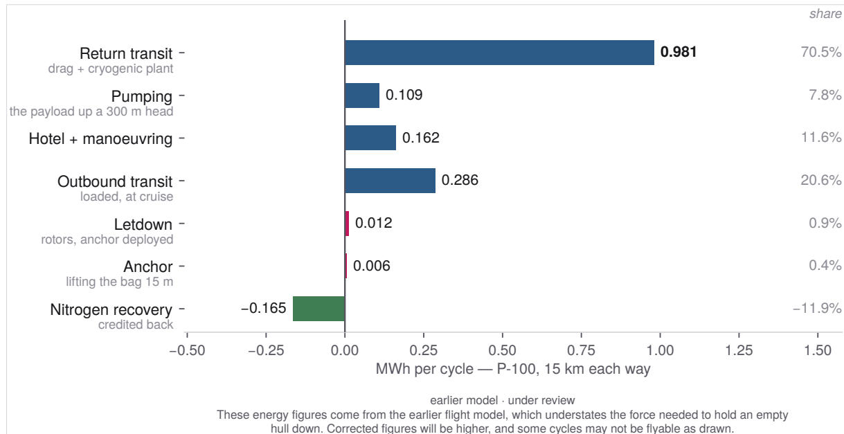
Figure 5. The reference ship's cycle ledger, printed from the model rather than transcribed. Three quarters of it is the return leg; the anchor is the smallest positive line and it is the reason the letdown is the second smallest.
