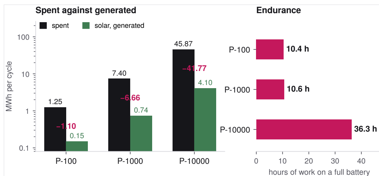
Figure 5. Spend against generation, and endurance on a full battery. This is the project's central public conclusion and it is not a favourable one.
