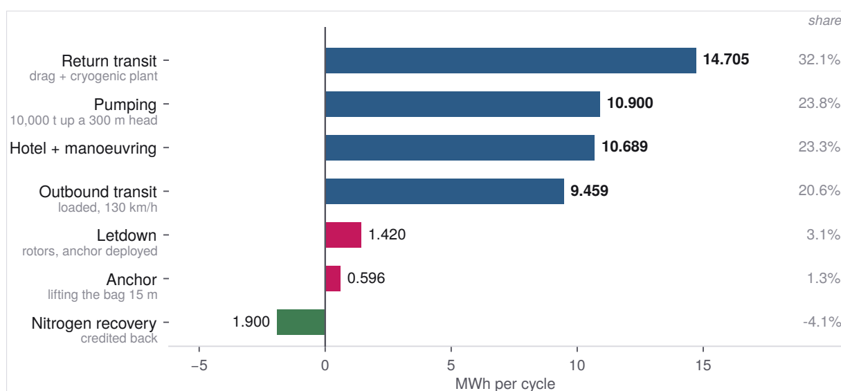
Figure 4. The cycle ledger, printed from the model. Seventy-six per cent of it is transit and pumping; the mechanism that closes the descent costs 1.3%.
