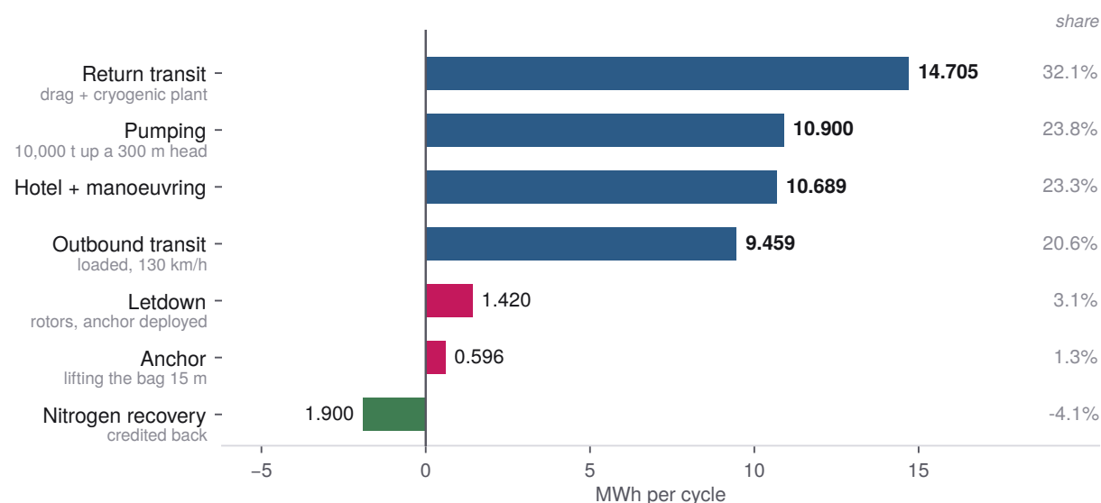
Figure 4. The cycle ledger, printed from the model. Seventy-six per cent of it is transit and pumping; the mechanism that closes the descent costs 1.3%.
