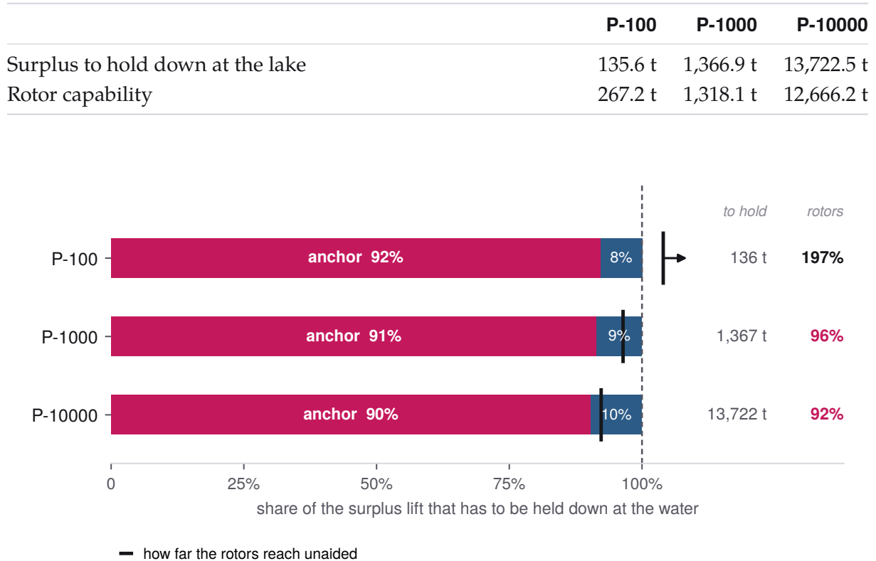
Figure 3. The problem the anchor solves. The bar is what has to be held down at the water; the tick is how far the rotors reach unaided.
