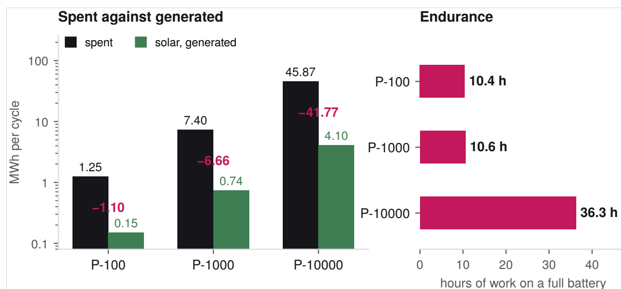
Figure 7. What each hull spends against what its skin makes, and how long a full battery lasts.
