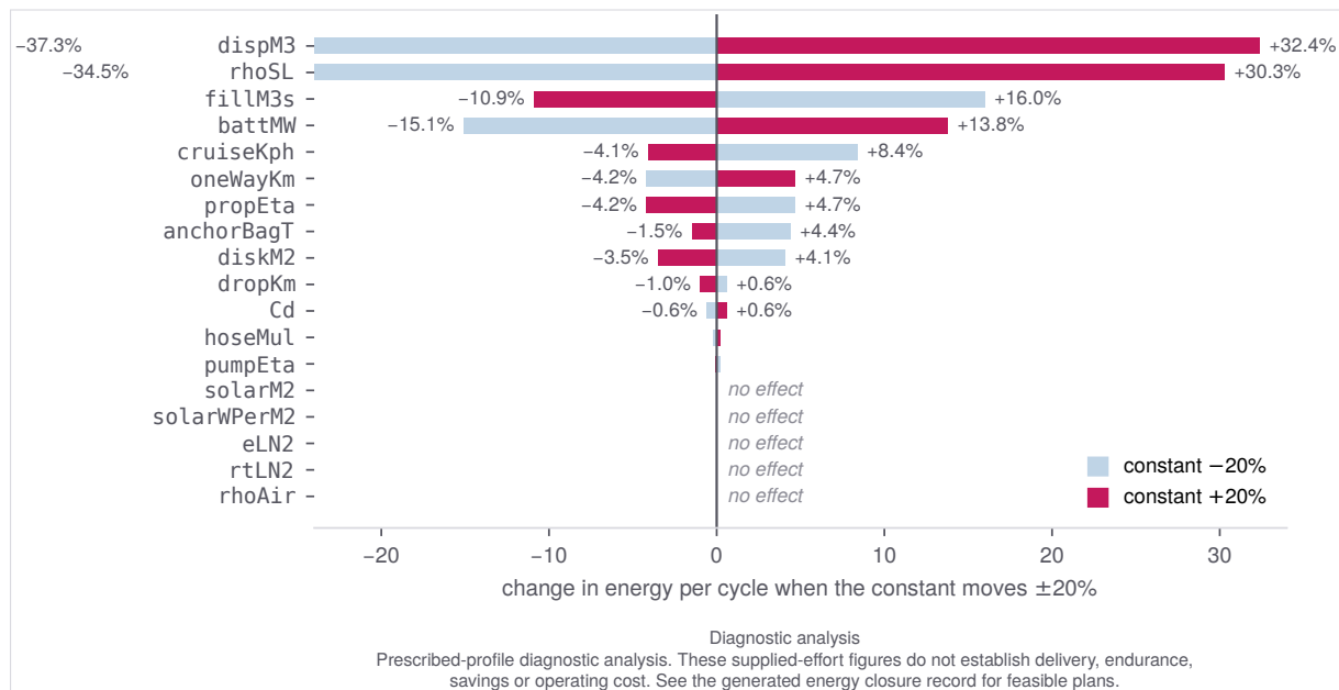
Figure 8. Every constant moved \pm 20\% , measured rather than asserted. The top of the table is aerodynamics and speed; the two constants corrected on 2026-08-09 now move the headline by 0.8% and 0.0%.
