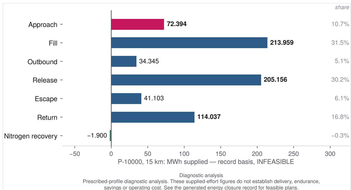
Figure 6. The same ledger at the limit case. The proportions invert: pumping and water handling dominate where flying did, which is the square-cube law seen from the other side.
