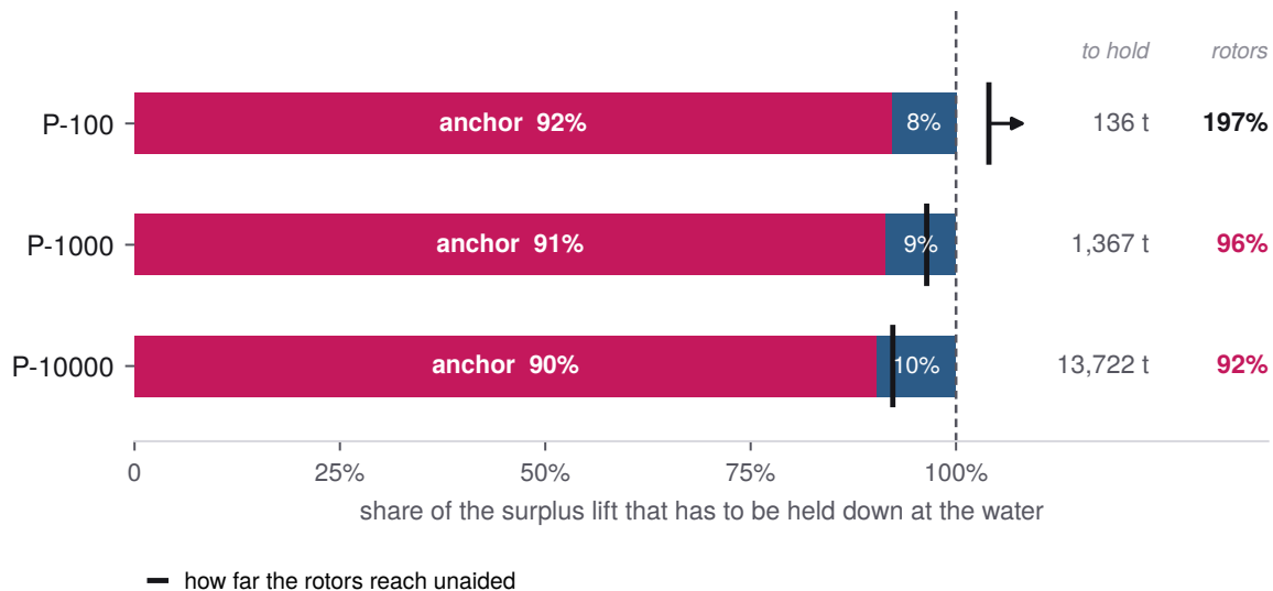
Figure 3. What has to be held down at the water, and what holds it. The bar is the job; the tick is how far the rotors reach unaided.
