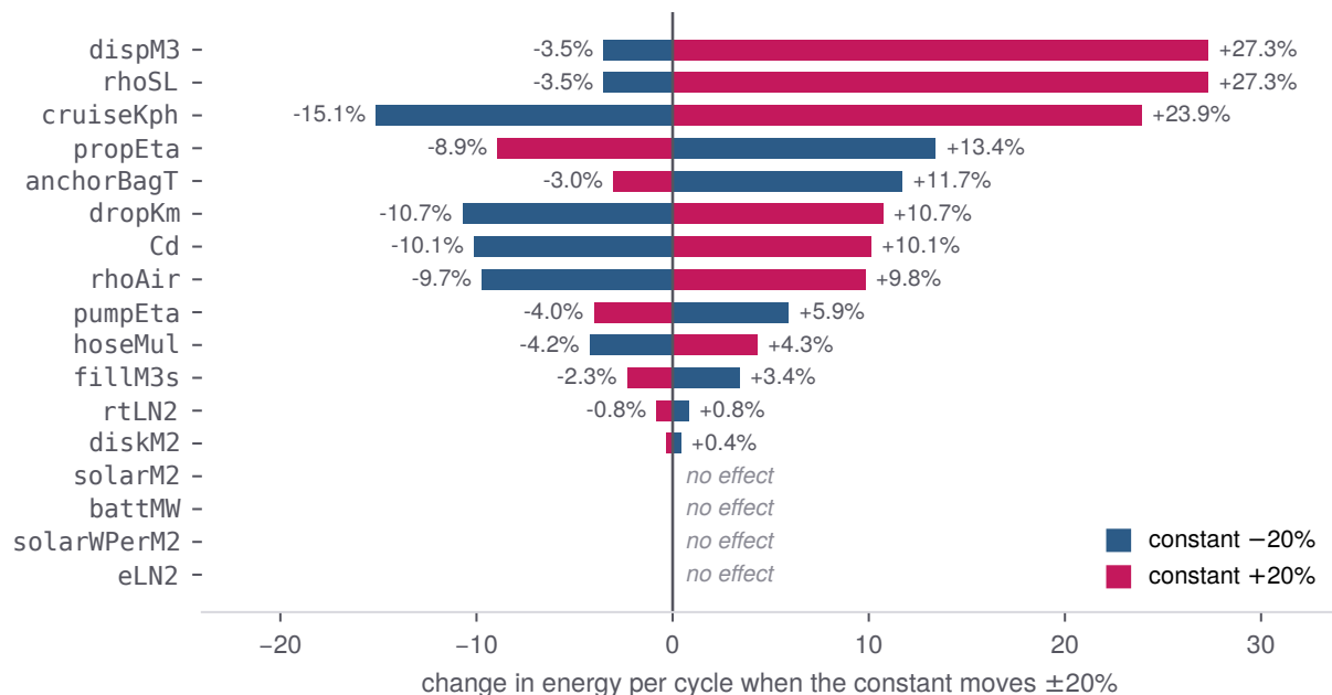
Figure 6. Every constant moved \pm 20\% , measured rather than asserted. The top of the table is aerodynamics and speed; the two constants corrected on 2026-08-09 now move the headline by 0.8% and 0.0%.
