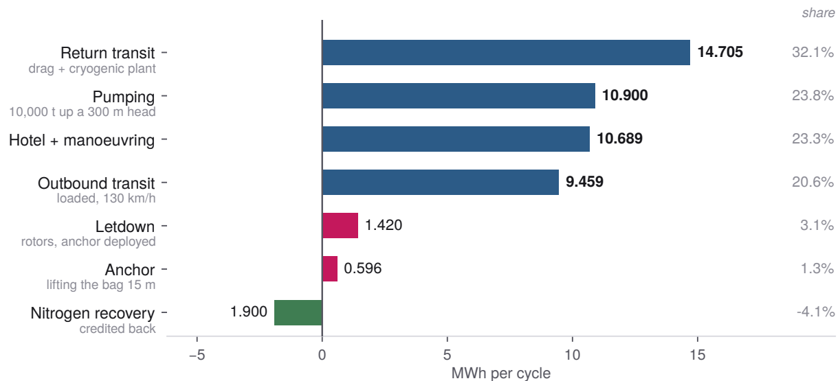
Figure 4. The cycle ledger, printed from the model rather than transcribed. The anchor is the smallest positive line, and it is the reason the letdown is the second smallest.
