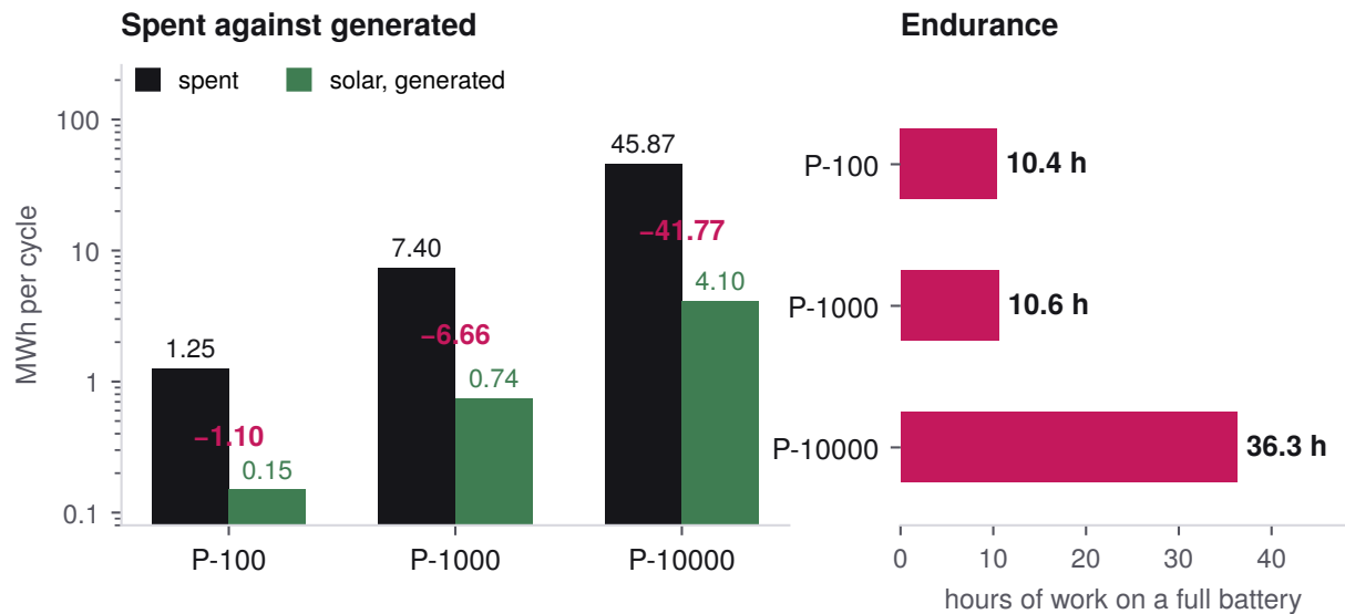
Figure 5. What each hull spends against what its skin makes, and how long a full battery lasts.
