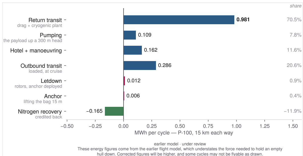
Figure 4. The reference ship's cycle ledger, printed from the model. Three quarters of it is the return leg; the mechanism that closes the descent costs half a per cent.
