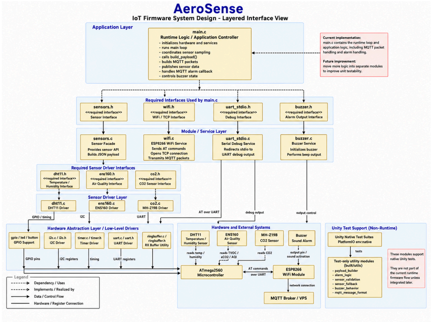
Figure 4 – IoT Firmware System Design – Layered Interface View
