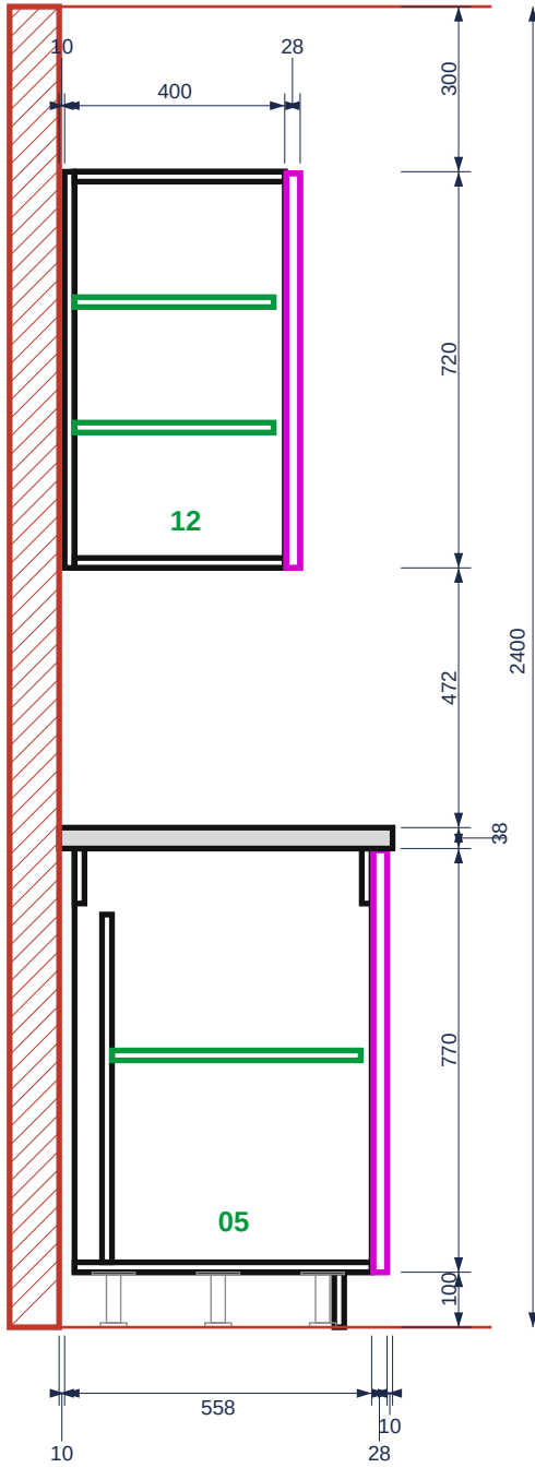
SECTION B-B · through units 05 and 12 looking along the wall, towards its start
