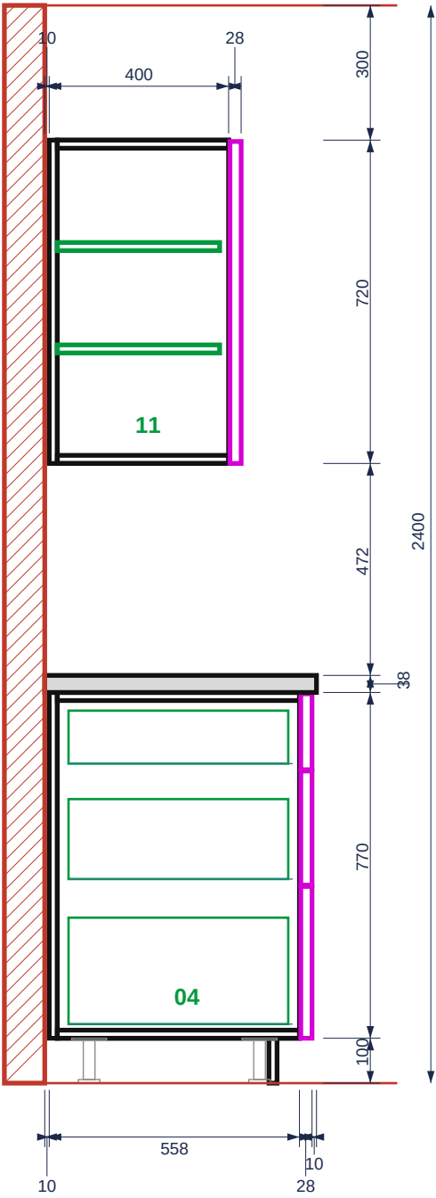
SECTION A-A · through units 04 and 11 looking along the wall, towards its start
