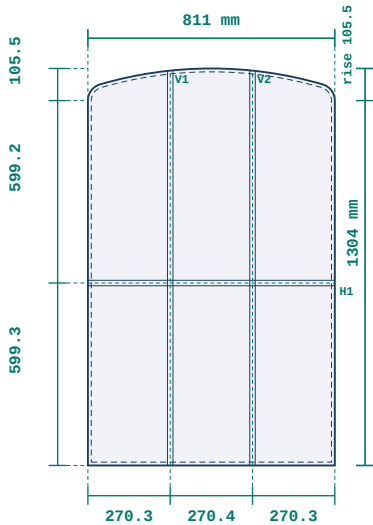
2 · TC-BARS — ARCHED LEAF GLASS double 4x16x4 · toughened · Standard · Argon · clear · spacer: silver (warm edge) · bars: 1H x 2V astragal · arched · R 55.5/1305.5 · rise 105.5 · springing 1198.5
