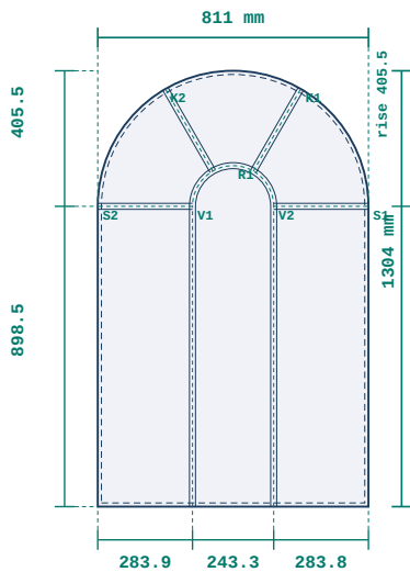
1 · SEMI-HUB — ARCHED LEAF GLASS double 4x16x4 · toughened · Standard · Argon · clear · spacer: silver (warm edge) · bars: hub-spoke astragal · arched · R 405.5 · rise 405.5 · springing 898.5
