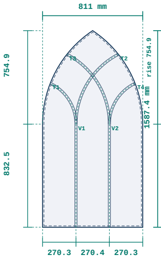
3 · GOTHIC-X — ARCHED LEAF GLASS double 4x16x4 · toughened · Standard · Argon · clear · spacer: silver (warm edge) · bars: intersecting astragal · arched · R 905.5 · rise 754.9 · springing 832.5
