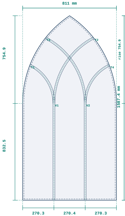
3 · GOTHIC-X — ARCHED LEAF GLASS double 4x16x4 · toughened · Standard · Argon · clear · spacer: silver (warm edge) · bars: intersecting astragal · arched · R 905.5 · rise 754.9 · springing 832.5
