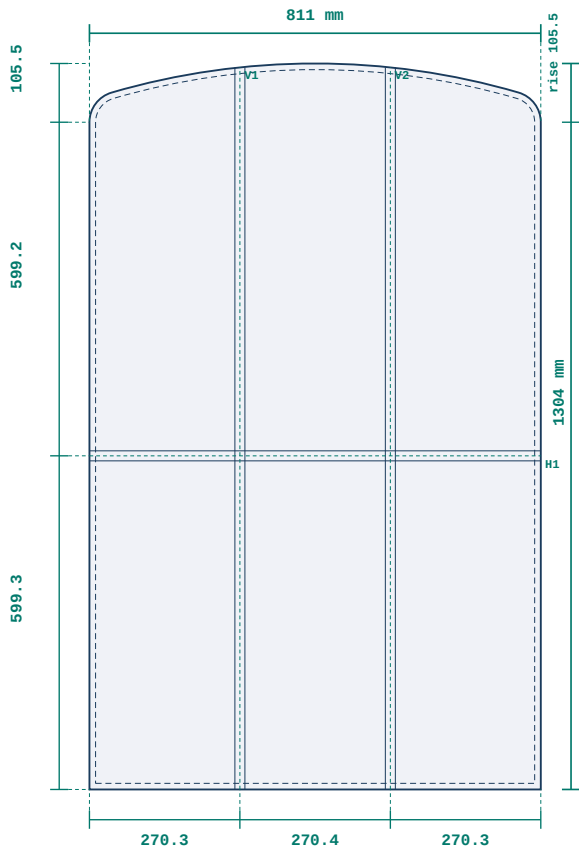
2 · TC-BARS — ARCHED LEAF GLASS double 4x16x4 · toughened · Standard · Argon · clear · spacer: silver (warm edge) · bars: 1H x 2V astragal · arched · R 55.5/1305.5 · rise 105.5 · springing 1198.5
