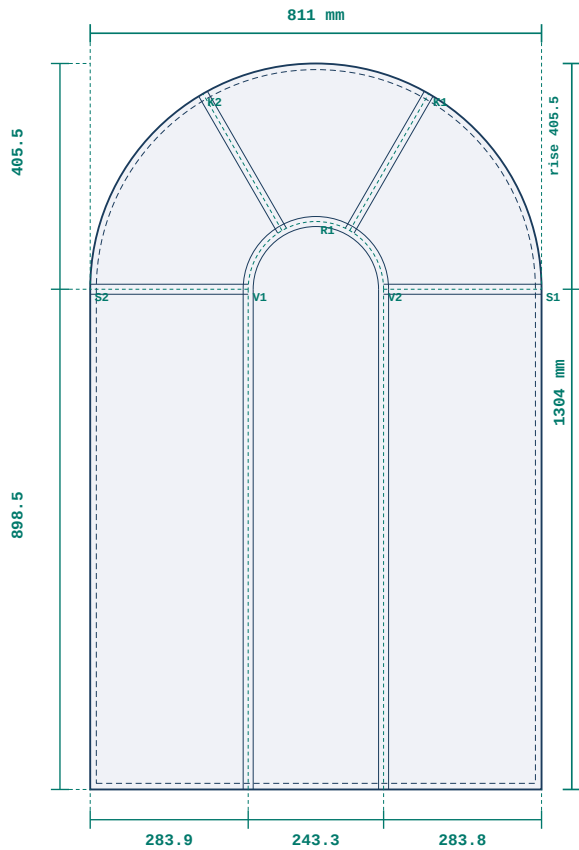
1 · SEMI-HUB — ARCHED LEAF GLASS double 4x16x4 · toughened · Standard · Argon · clear · spacer: silver (warm edge) · bars: hub-spoke astragal · arched · R 405.5 · rise 405.5 · springing 898.5
