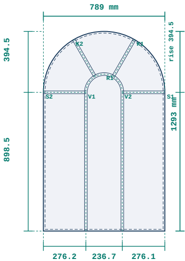
1 · SEMI-HUB — ARCHED LEAF GLASS double 4x16x4 · toughened · Standard · Argon · clear · spacer: silver (warm edge) · bars: hub-spoke astragal · arched · R 394.5 · rise 394.5 · springing 898.5
