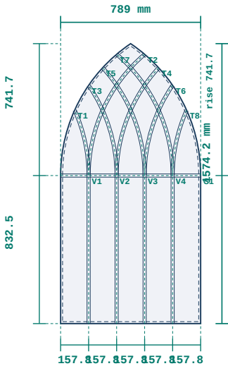
3 · GOTHIC-X — ARCHED LEAF GLASS double 4x16x4 · toughened · Standard · Argon · clear · spacer: silver (warm edge) · bars: intersecting astragal · arched · R 894.5 · rise 741.7 · springing 832.5
