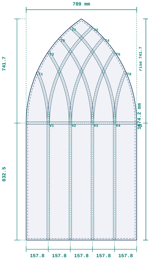
3 · GOTHIC-X — ARCHED LEAF GLASS double 4x16x4 · toughened · Standard · Argon · clear · spacer: silver (warm edge) · bars: intersecting astragal · arched · R 894.5 · rise 741.7 · springing 832.5
