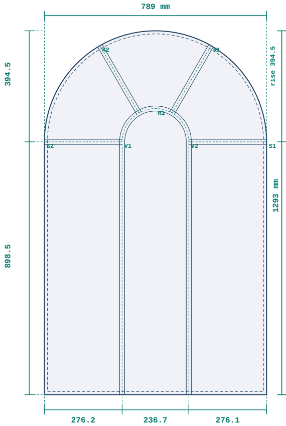
1 · SEMI-HUB — ARCHED LEAF GLASS double 4x16x4 · toughened · Standard · Argon · clear · spacer: silver (warm edge) · bars: hub-spoke astragal · arched · R 394.5 · rise 394.5 · springing 898.5
