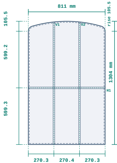
2 · TC-BARS — ARCHED LEAF GLASS double 4x16x4 · toughened · Standard · Argon · clear · spacer: silver (warm edge) · bars: 1H × 2V astragal · arched · R 55.5/1305.5 · rise 105.5 · springing 1198.5
