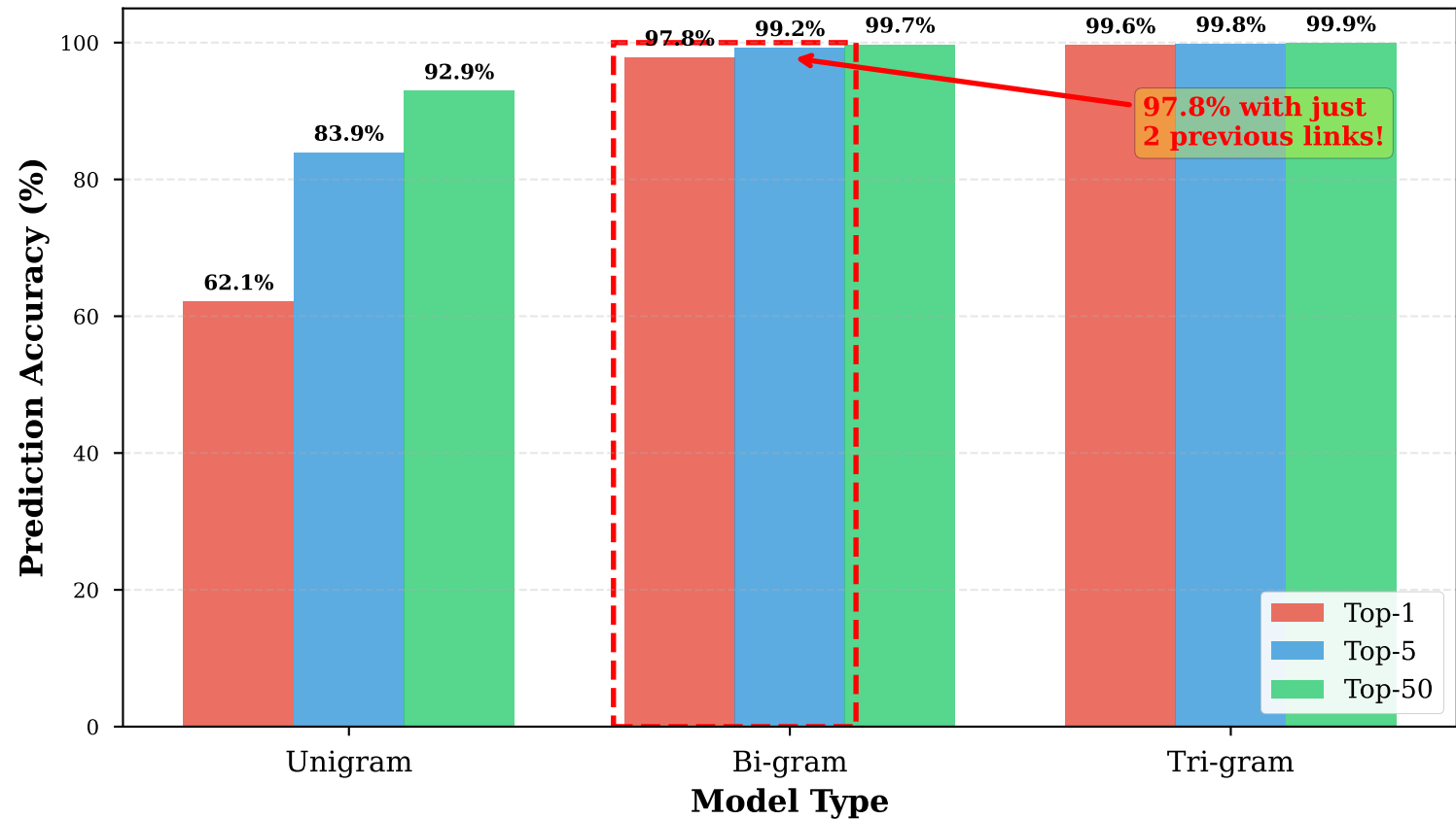
Figure 2: Link Prediction Accuracy by Context Size
