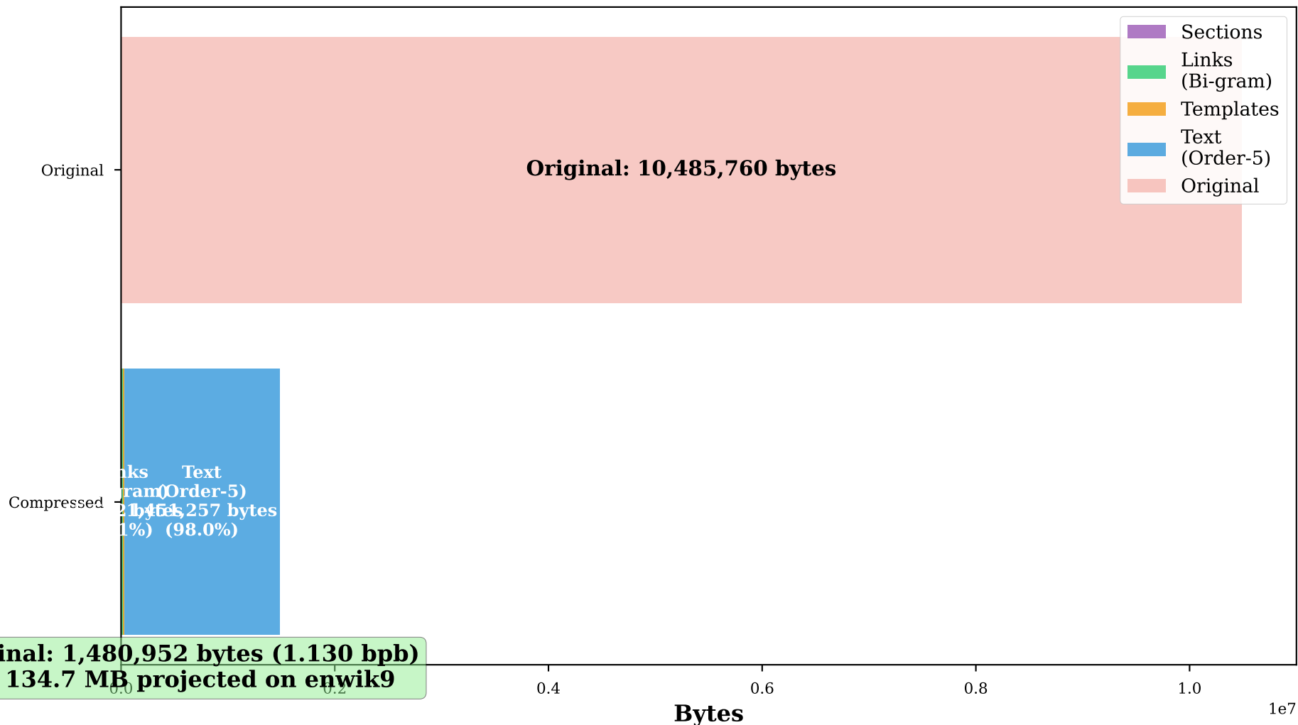
Figure 5: Overall Document Compression Breakdown (10 MB test)
