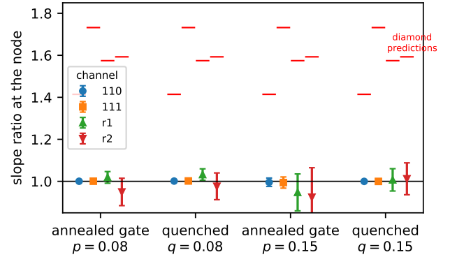
FIG. 1. Slope ratios at the node, gate and quenched rows at each q , against the factorized-transport (diamond) prediction. Error bars are leave-one-block-out jackknives over ten independent medium blocks with the same- q gate-row systematic added in quadrature. [MEASURED]
