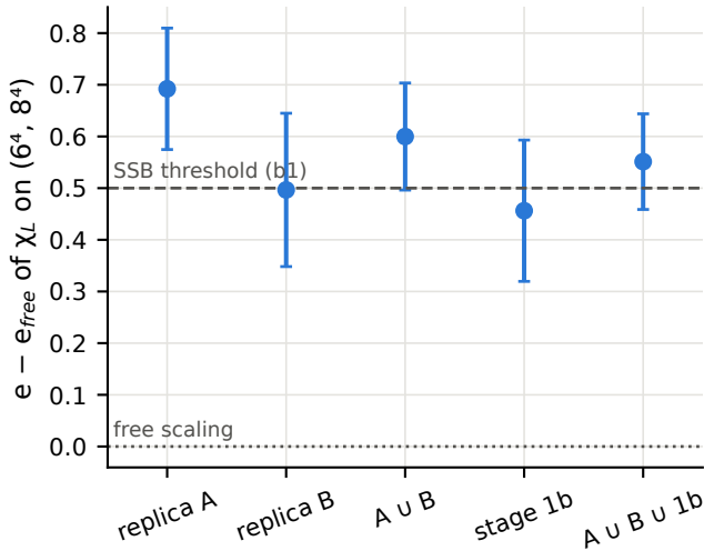
SMG ( y = 3.0 ), h = 2 : light pair susceptibility
