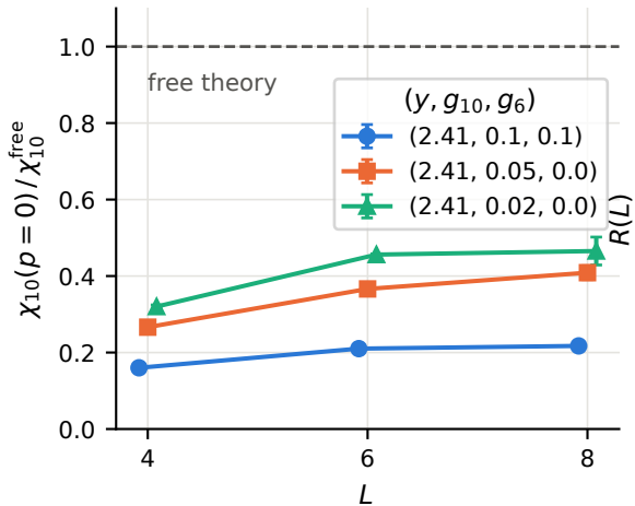
(a) complete 10-channel correlator at P_c
