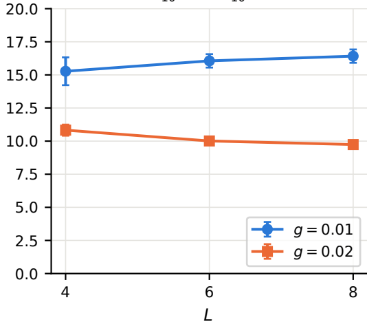
(b) R = [\chi_{10}^{\text{wedge}} - \chi_{10}^{\text{compl}}]/g at P_c
