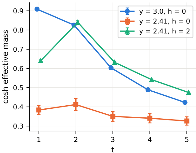
6^3 \times 12 : light pair channel, no plateau
