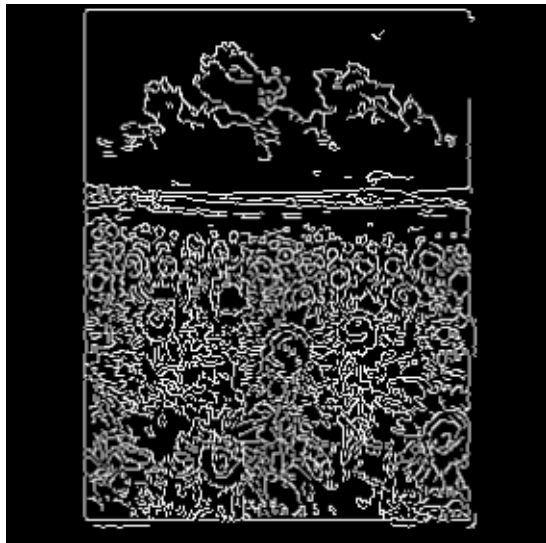
Canny 100/200
