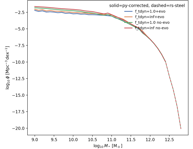
Paper 1 Fig. 8 style -- satellite SMF, frozen model, f_{\text{tdyn}} \times \text{SMHM} -evolution sweep (G15)
