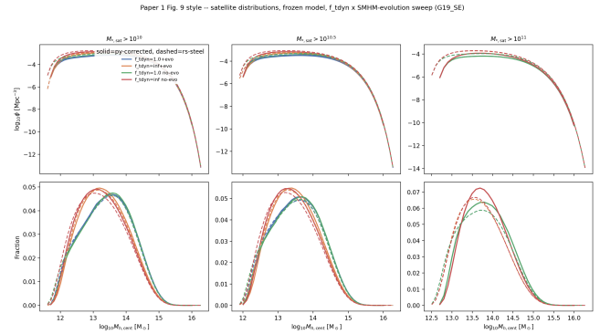
Figure 3. Satellite number density (top row) and fractional distribution (bottom row, eq. 16 of Paper 1) vs. parent halo mass under the same frozen-model f_{\text{tdyn}} \times SMHM-evolution sweep as Fig. 2 (Paper 1 Fig. 9), for three increasing satellite stellar-mass cuts (columns). Four lines, two implementations.
