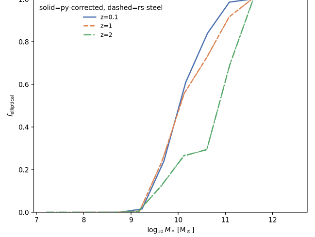
Paper 2 Fig. 11 style -- elliptical fraction from major-merger history (G18) ( f = 1 - \exp(-N_{\text{major}}) , an interpretation -- see script docstring)
