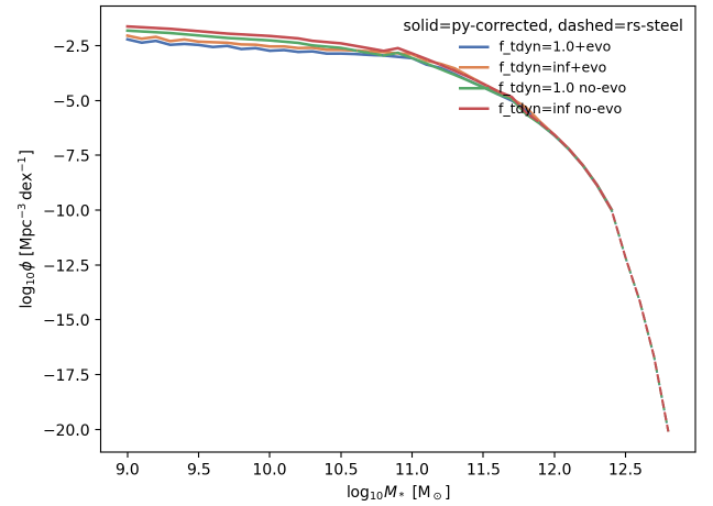
Figure 2. Frozen-model satellite stellar mass function under the f_{\text{tdyn}} \times SMHM-evolution sweep that Paper 1 §4.1 actually uses (not a stellar-population comparison, which is a different figure in the same paper). Four lines, two implementations.
