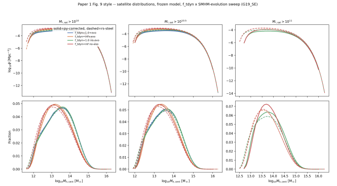
Figure A2. Satellite number density (top row) and fractional distribution (bottom row, eq. 16 of Paper 1) vs. parent halo mass under the same frozen-model f_{\text{tdyn}} \times \text{SMHM} -evolution sweep as Fig. A1 (Paper 1 Fig. 9), for three increasing satellite stellar-mass cuts (columns). Four lines, two implementations.
