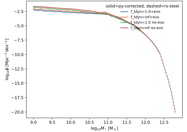
Figure A1. Frozen-model satellite stellar mass function under the f_{\text{tdyn}} \times \text{SMHM} -evolution sweep that Paper 1 §4.1 actually uses (not a stellar-population comparison, which is a different figure in the same paper). Four lines, two implementations.
