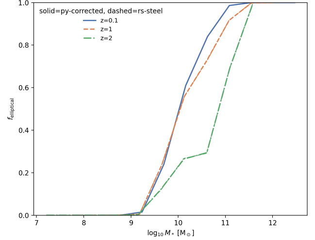
Paper 2 Fig. 11 style -- elliptical fraction from major-merger history (G18) ( f = 1 - \exp(-N_{\text{major}}) , an interpretation -- see script docstring)
