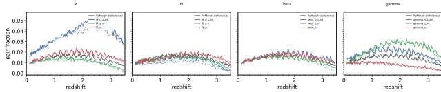
Paper 3 Fig. 3 style -- pair fraction vs. z , SMHM parameter sensitivity (solid=py-corrected, dashed=rs-steel)
