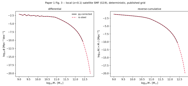
Figure 1. Local ( z \sim 0.1 ) satellite stellar mass function, deterministic mode, published grid: differential (left) and reverse-cumulative (right). Solid: py-corrected . Dashed: rs-steel .
