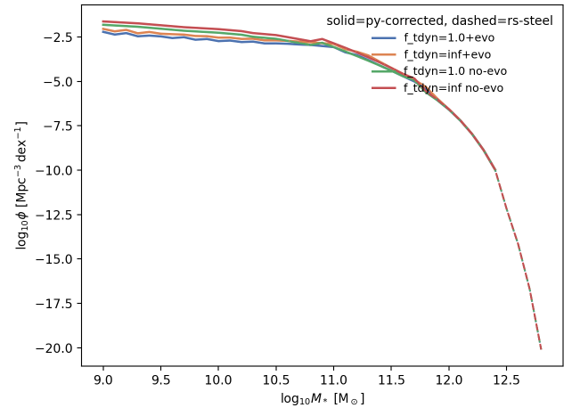
Figure 2. Frozen-model satellite stellar mass function under the f_{\text{tdyn}} \times \text{SMHM} -evolution sweep that Paper 1 §4.1 actually uses (not a stellar-population comparison, which is a different figure in the same paper). Four lines, two implementations.
