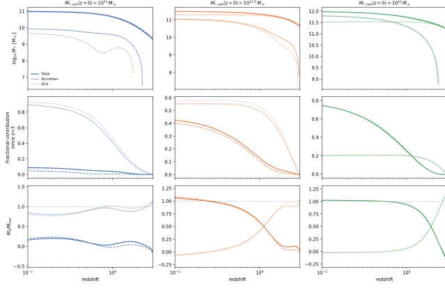
Paper 2 Fig. 8 style -- mass track decomposition (cmodel) (solid=py-corrected, dashed=rs-steel)
