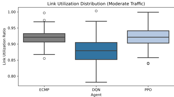
Figure 5. Link Utilization Distribution (Moderate Traffic).
