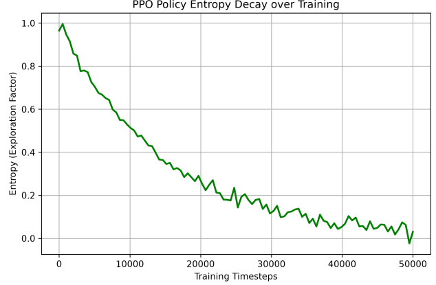
Figure 11. PPO Policy Entropy Decay over 50,000 Training Timesteps.
