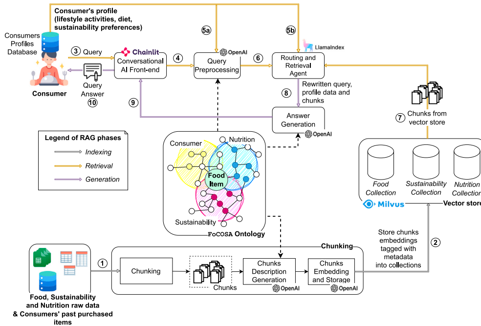
Fig. 4. Proposed ontology-enhanced RAG architecture of the conversational food advisory system. In the figure, three dashed arrows highlight the steps of RAG where the FoCOSA ontology has been employed.
