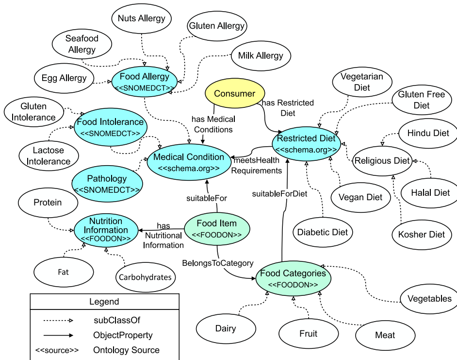
Fig. 2. Ontological concepts and relationships of the Nutrition module of the FoCOSA ontology.
