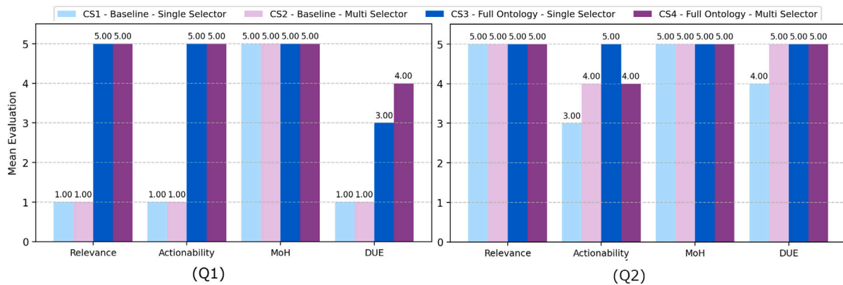
Fig. 7. Excerpt of quality criteria scores detailed for query Q1 (left) and Q2 (right).
