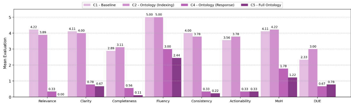
Fig. 8. Average quality criteria scores over configurations C1, C2, C4, and C5 using DeepSeek-R1 (14B) with Nomic embeddings.
