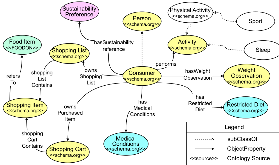
Fig. 1. Ontological concepts and relationships of the Consumer module in the FoCOSA ontology.
