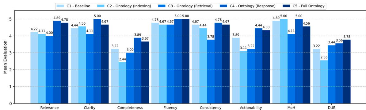
Fig. 5. Average quality criteria scores over the different configurations C1 to C5 (Single Selector).
