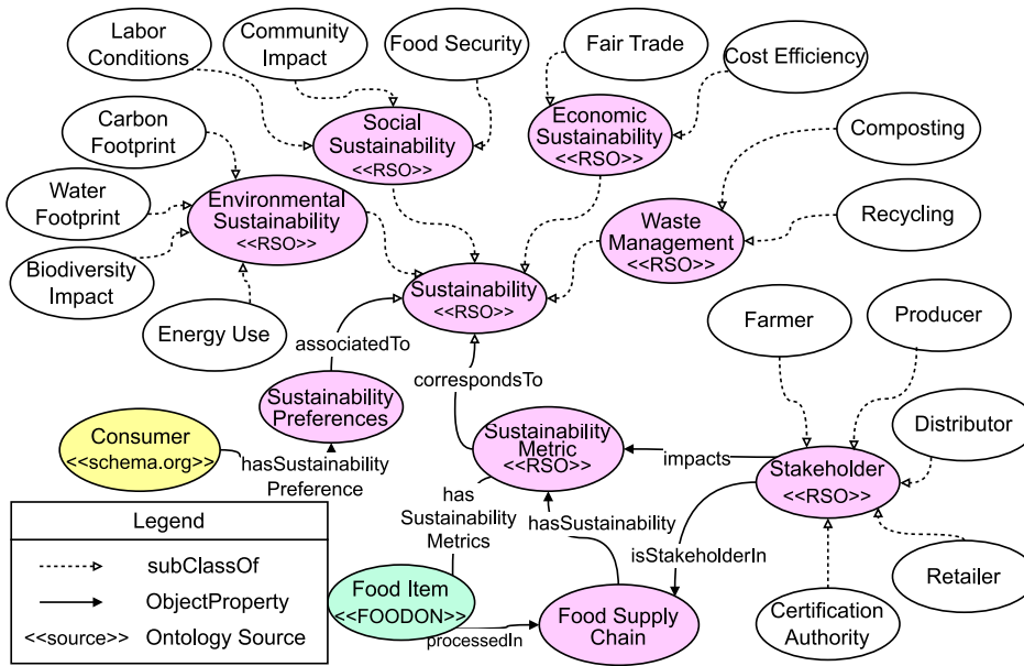
Fig. 3. Ontological concepts and relationships of the Sustainability module of the FoCOSA ontology.
