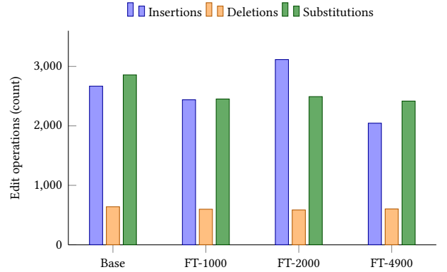
Figure 3: Edit operations per system. FT-4900 wins mainly by cutting insertions; FT-2000 loses its gains to an insertion increase.
