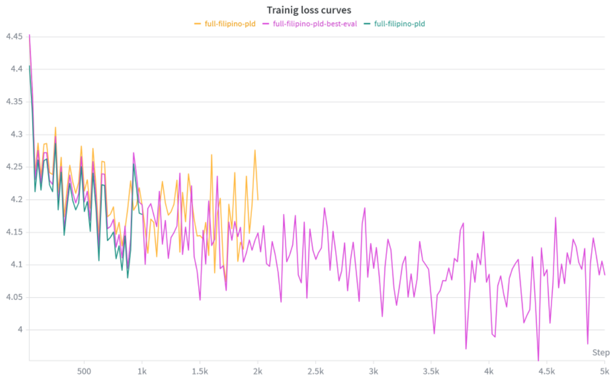
Figure 4: Combined W&B training-loss curves for the Filipino OmniVoice fine-tuning runs.
