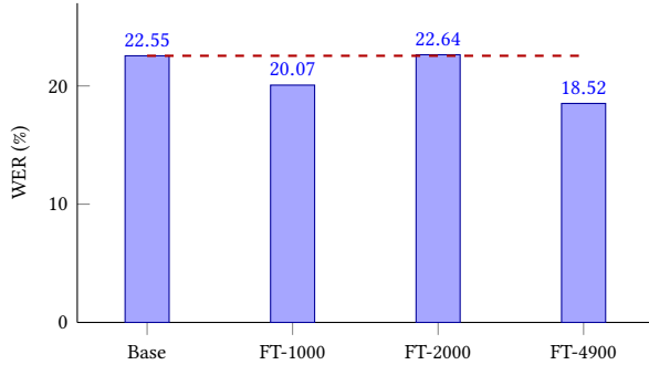
Figure 2: Test-set WER by system. The dashed line marks the base-model WER; only FT-1000 and FT-4900 fall below it.
