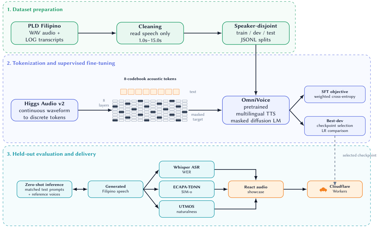
Figure 1: System architecture for Filipino OmniVoice fine-tuning, evaluation, and public showcase delivery.
