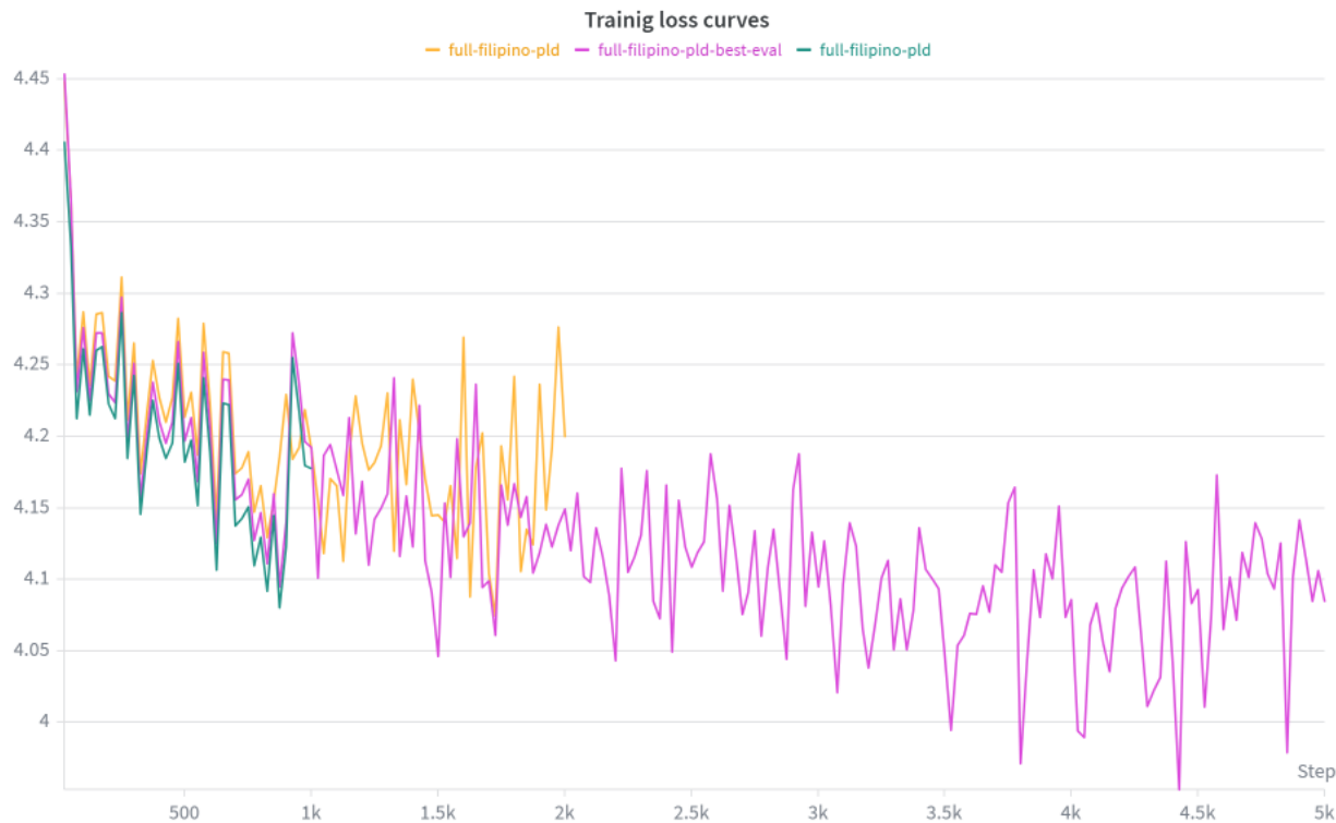
Figure 5: Combined W&B training-loss curves for the Filipino OmniVoice fine-tuning runs, including the preliminary exploratory runs.
