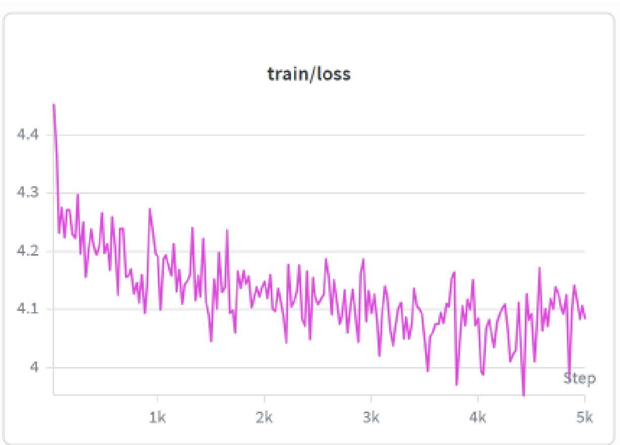
Figure 6: W&B run screenshot for the 5000-step fine-tuning run at learning rate 1e-5 , whose best-development-loss checkpoint (step 4900) is the recommended model.
