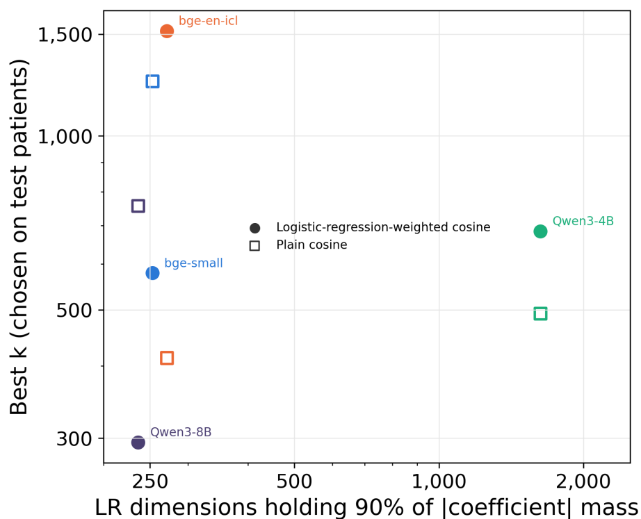
Figure 6. Logistic-regression dimensions against best k for the 4 encoders. The horizontal axis is the fewest embedding dimensions
