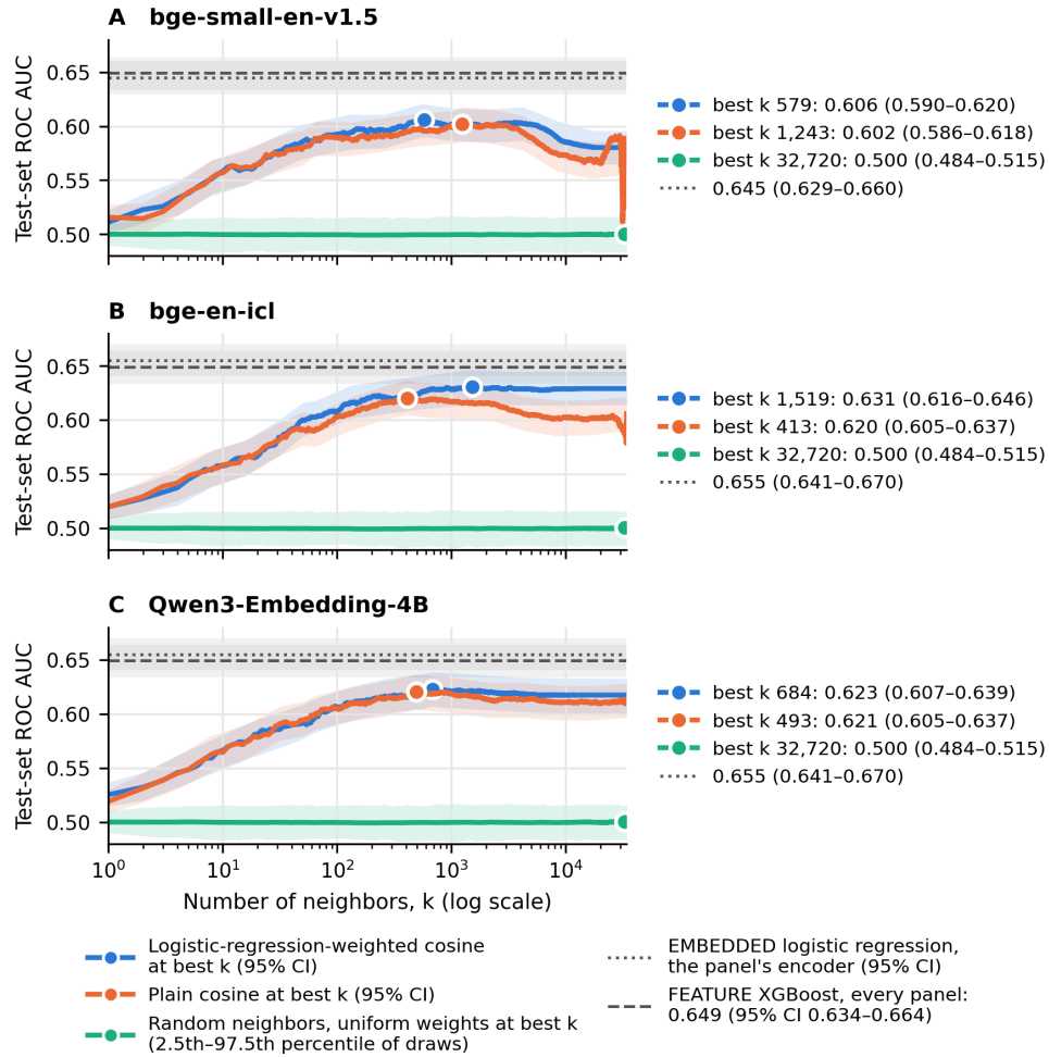
Figure 5. Retrieval discrimination by neighborhood size for the other 3 encoders: (A) bge-small-en-v1.5, (B) bge-en-icl, and (C) Qwen3-Embedding-4B. Figure 4 is the same plot for Qwen3-Embedding-8B. Each panel draws ROC AUC in 8,516 test patients at every k from 1 to 34,063 for logistic-regression-weighted and plain cosine retrieval,
