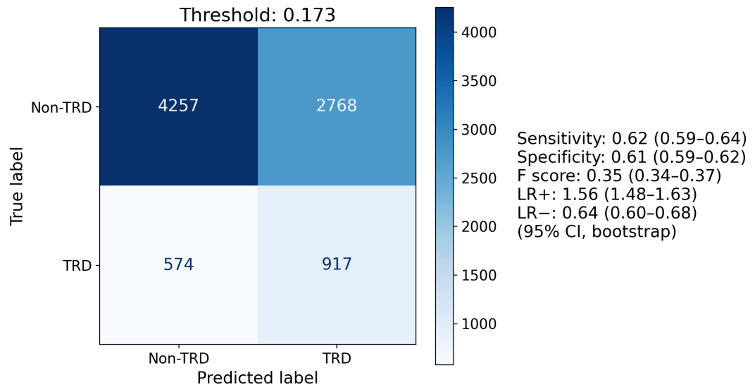
Figure S13. Confusion matrices at test-selected Youden J thresholds for embedded logistic regression (A) and feature-vector XGBoost (B). TRD refers to the treatment-switching proxy.
