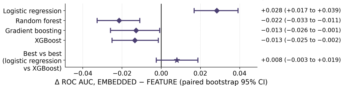
(B) Paired head-to-head difference, same held-out patients
