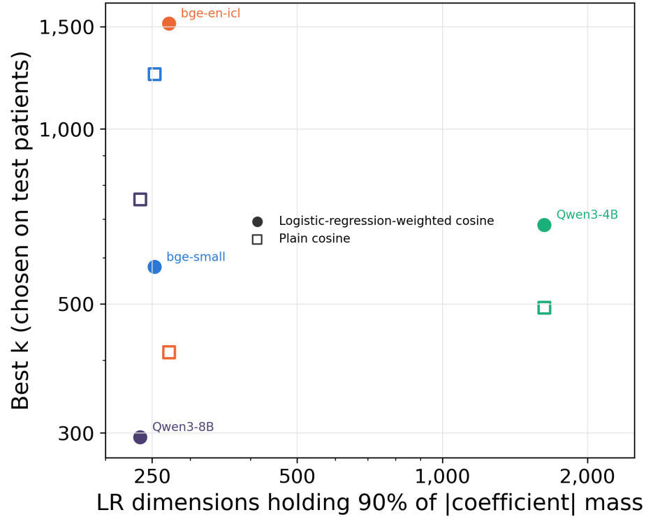
Figure 6. Logistic-regression dimensions against best k for the 4 encoders. The horizontal axis is the fewest embedding dimensions holding 90% of the absolute coefficient mass of each encoder’s embedded logistic regression. The vertical axis is the best k of logistic-regression-weighted (filled markers) and plain cosine retrieval (open markers), chosen on the test patients and therefore optimistic. Both axes are logarithmic.
