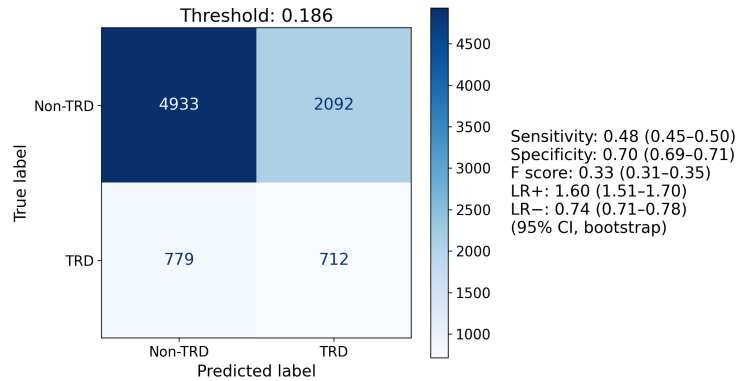
B Qwen3-Embedding-8B, plain-cosine nearest retrieval, k = 757
