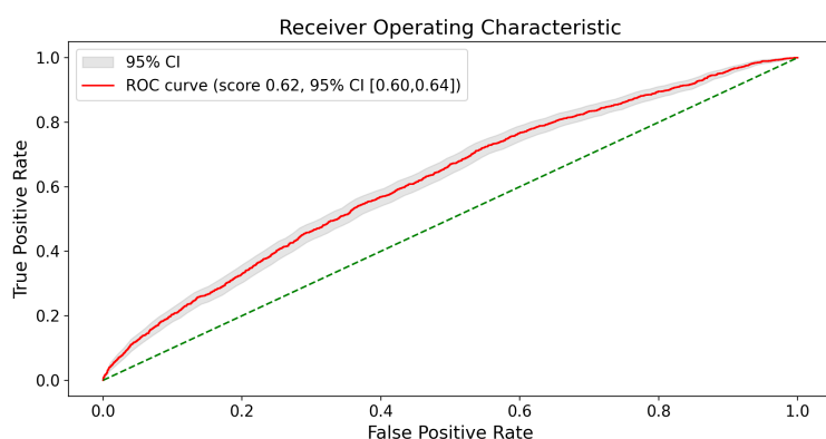
Figure S8. ROC curves at each arm's own test-selected best k, with \alpha = 1 for nearest retrieval. A-C: the primary encoder, Qwen3-Embedding-8B, under logistic-regression-weighted (A) and plain-cosine (B) nearest retrieval and uniform random retrieval (C). D-I: logistic-regression-weighted and plain-cosine nearest retrieval for bge-small-en-v1.5 (D-E), bge-en-icl (F-G), and Qwen3-Embedding-4B (H-I), each weighted by its own embedded logistic regression. C is the draw whose AUC at that k is closest to the mean of 1,000 draws. Best k was chosen on the test patients, so every panel is optimistic. Shaded bands are bootstrap 95% CIs. ROC: receiver operating characteristic.
