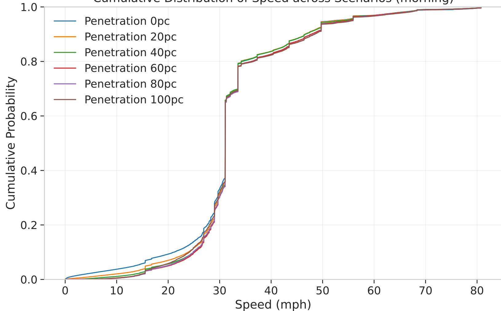
Cumulative Distribution of Speed across Scenarios (morning)
