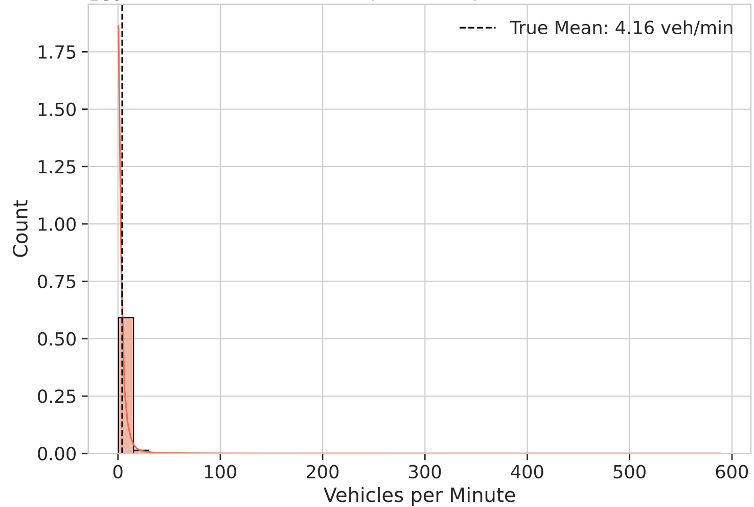
Flow Distribution (Active Only)
