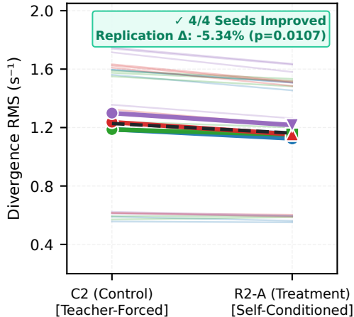
(b) Sample Divergence RMS (h=10)
