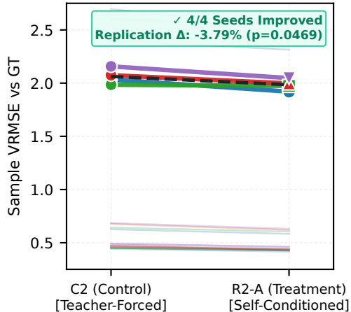
(a) Sample VRMSE (h=10)
