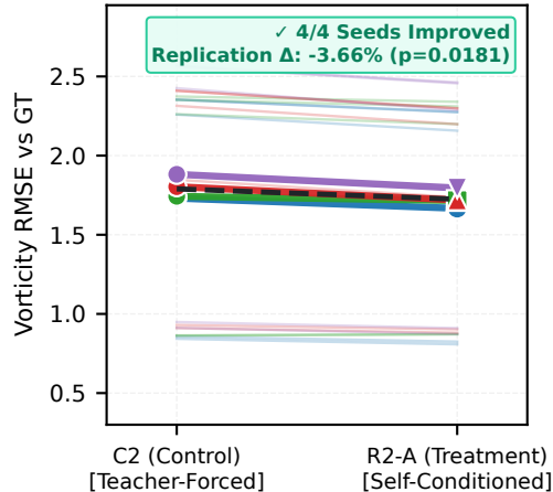
(c) Sample Vorticity RMSE (h=10)
