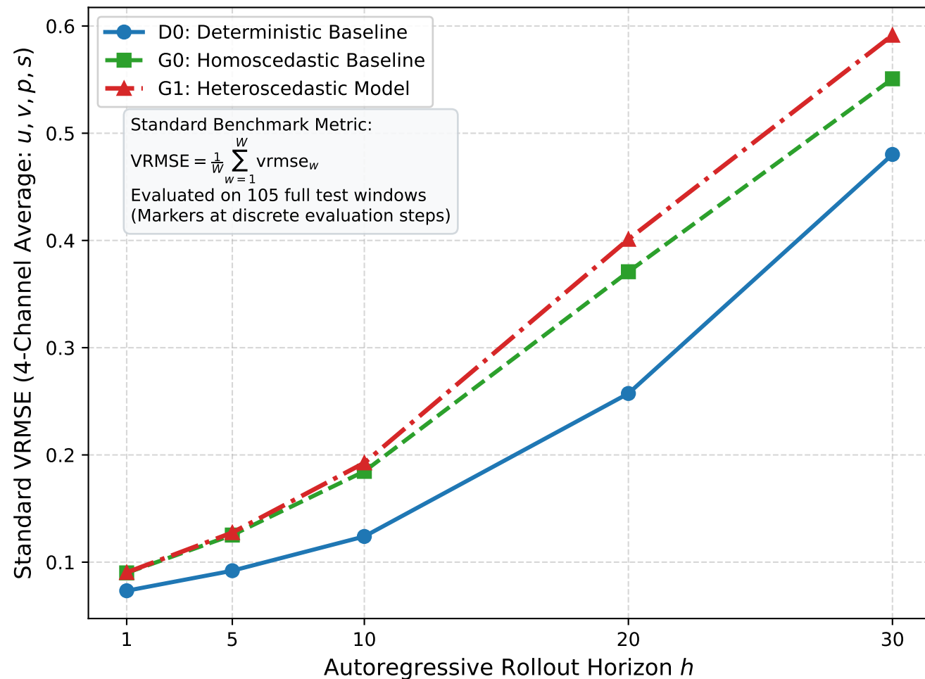
(a) Standard Benchmark VRMSE Evolution
