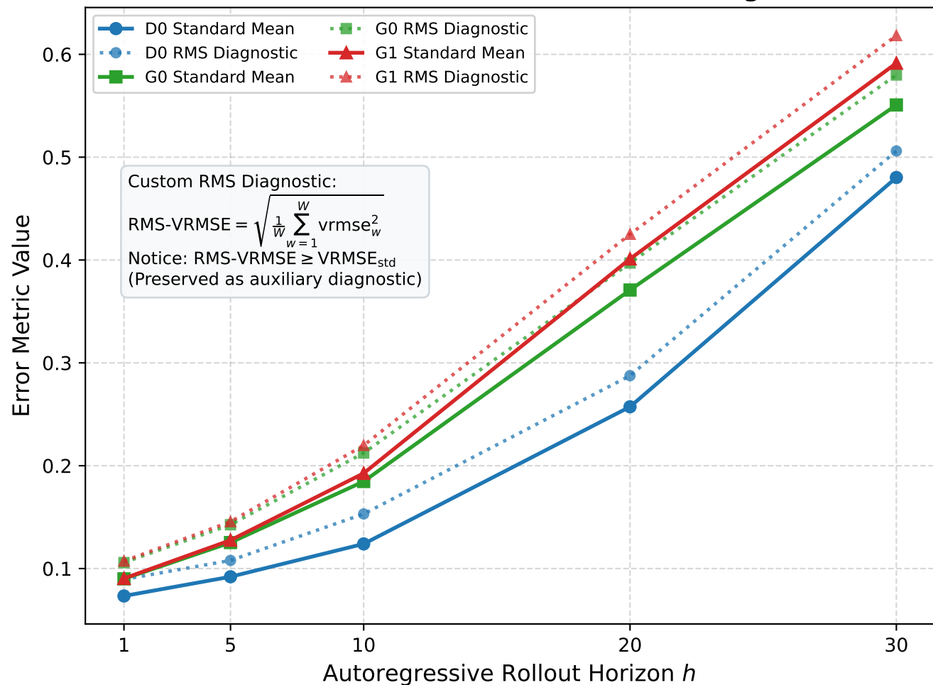
(b) Standard VRMSE vs. Custom RMS Diagnostic
