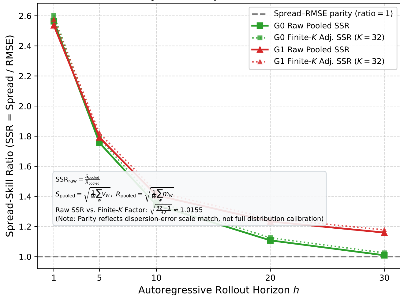
(b) Velocity Pooled Spread-Skill Ratio (SSR)
