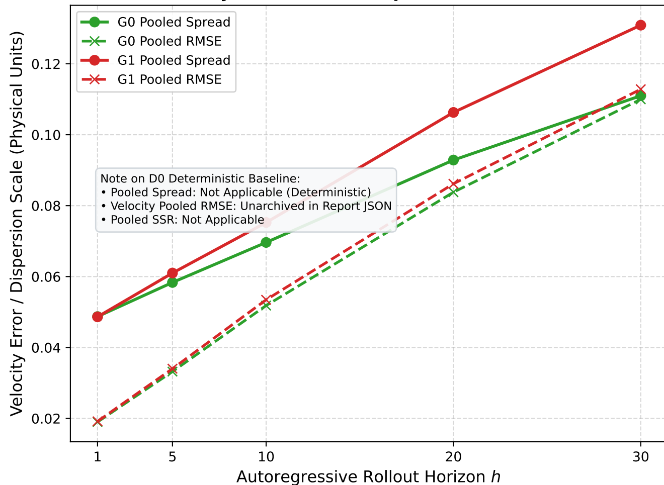
(a) Velocity Vector Pooled Spread vs. Pooled RMSE
