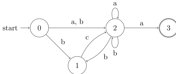
Figure 3: NFA for (a|b|bc)^+a
