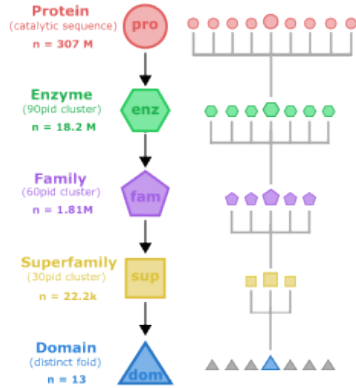
Fig 2C. PETadex Clustering
