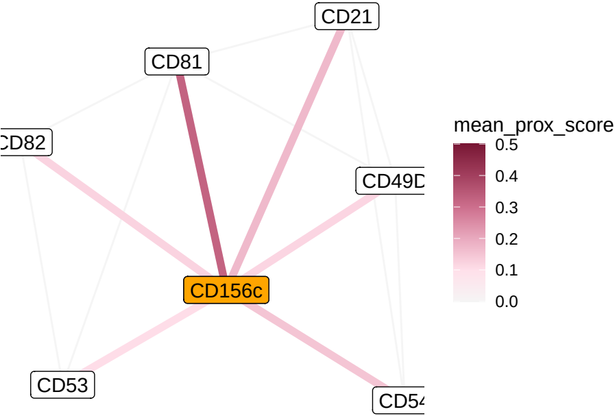
CD156c Interaction Network
