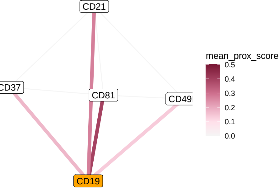
CD19 Interaction Network
