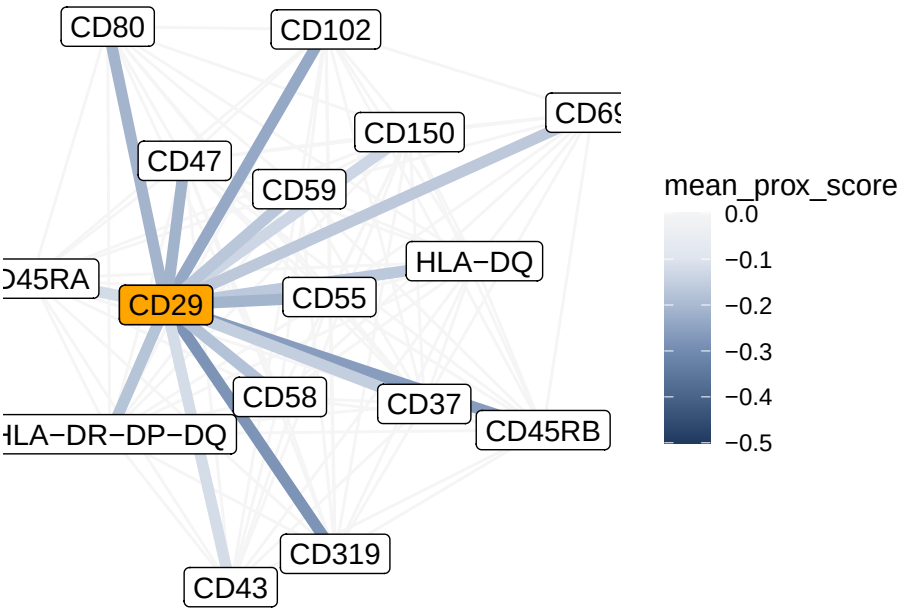
CD29 Interaction Network
