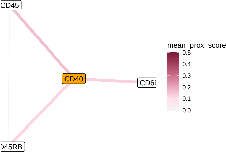
CD40 Interaction Network
