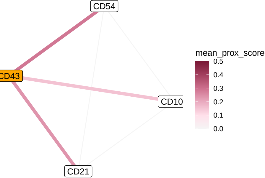
CD43 Interaction Network
